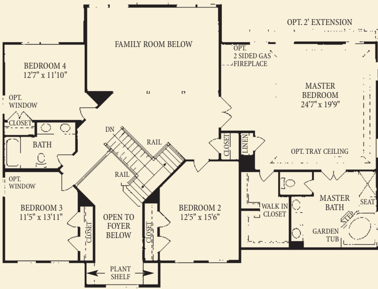
OPT. SECOND FLOOR PLAN - ELEVATION 1
